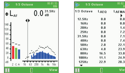
Figure 12. 1/3 Octave graph and list views
